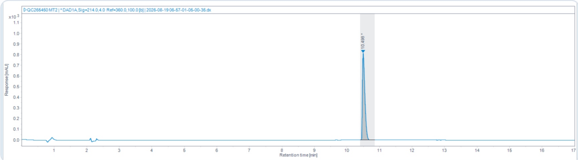
HPLC Chromatogram · Retention Time 10.498 min
